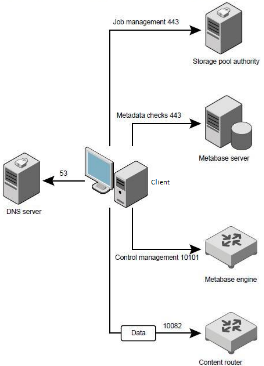
Figure 3-2 Communication ports
